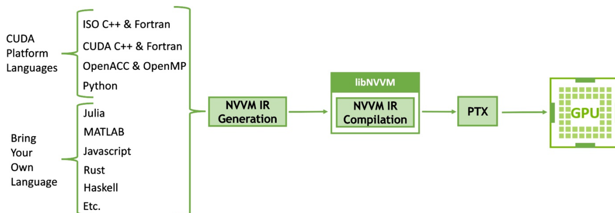
Figure 24. Compiling high-level Languages to PTX with libNVVM
