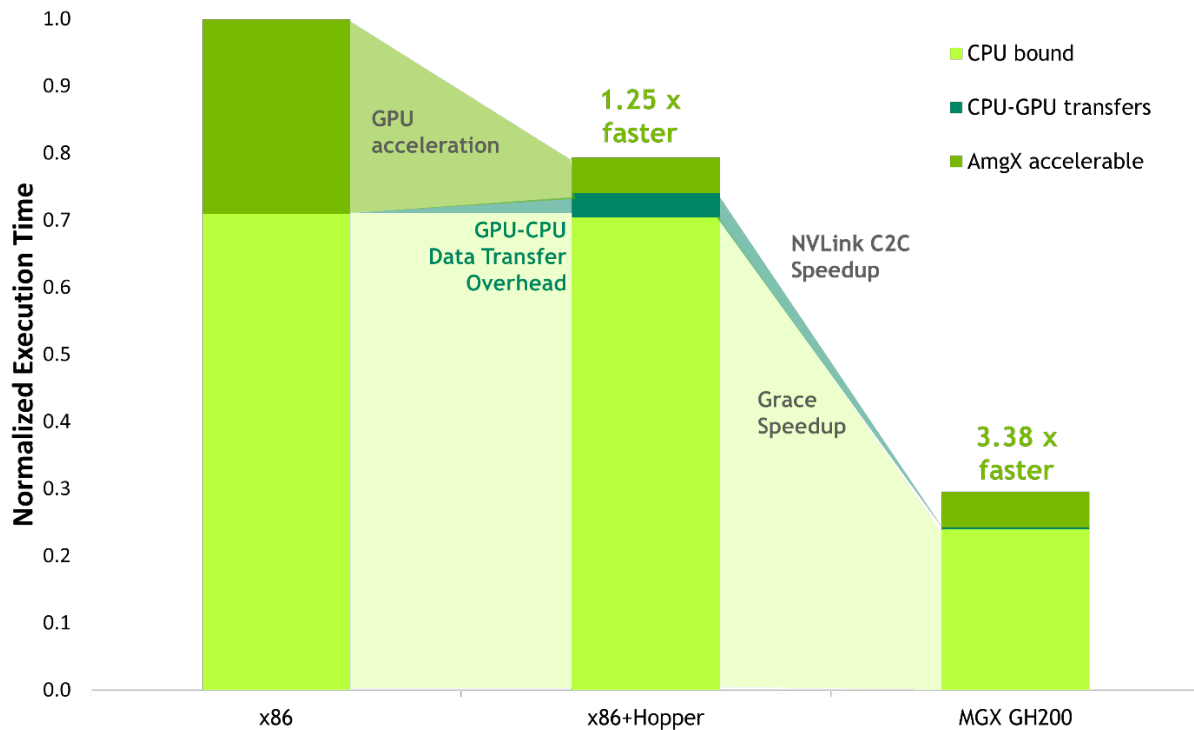
Figure 20. A performance simulation for OpenFOAM HPC Motorbike L (34 M cells) on MGX with GH200 with HBM3
