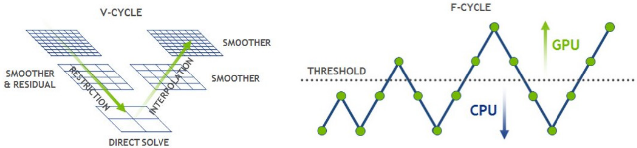
Figure 23. GH200 Simplifies Multigrid Linear Solvers
