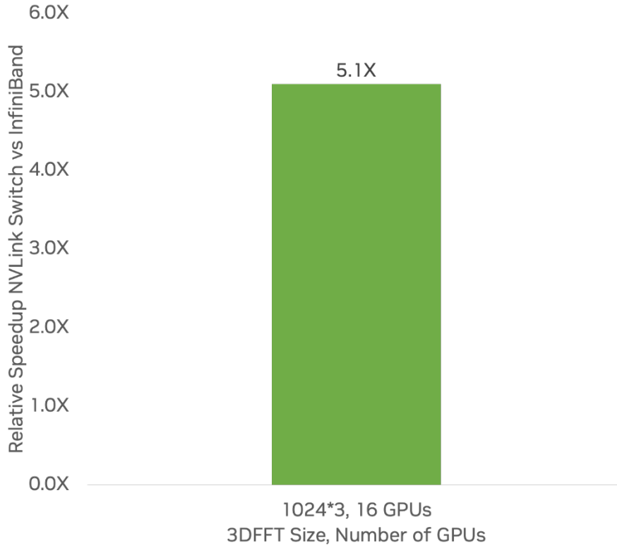
Figure 22. Speedup of GH200 NVL32 versus InfiniBand NDR400 on NVIDIA MGX with GH200 and HBM3 for 3D FFTs
