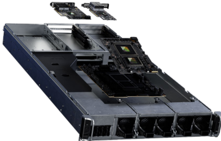
Figure 2. NVIDIA MGX Platform
