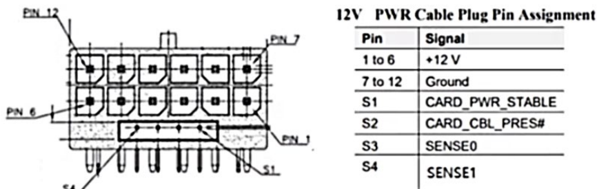
Figure 4-3. PCIe 16-Pin Power Connector Pin Assignment
